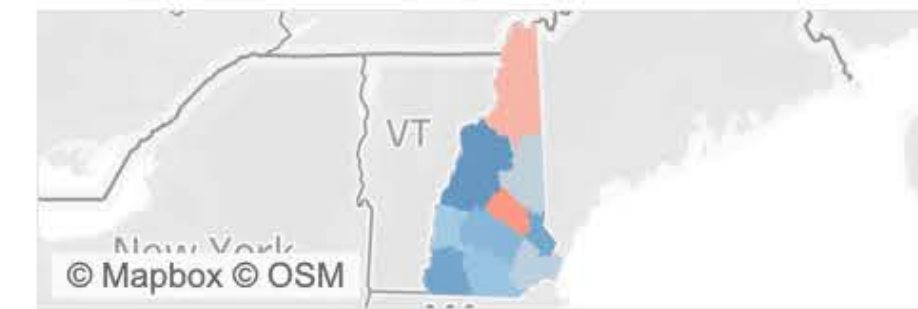
Senate Overperform 0
